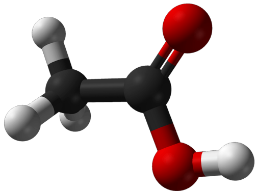
Acetic acid, \text{CH}_3\text{COOH}
