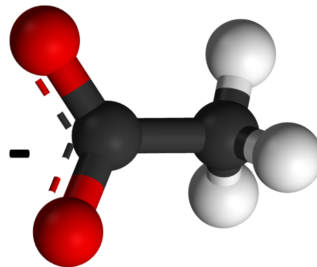
acetate ion, \text{CH}_3\text{COO}^-
